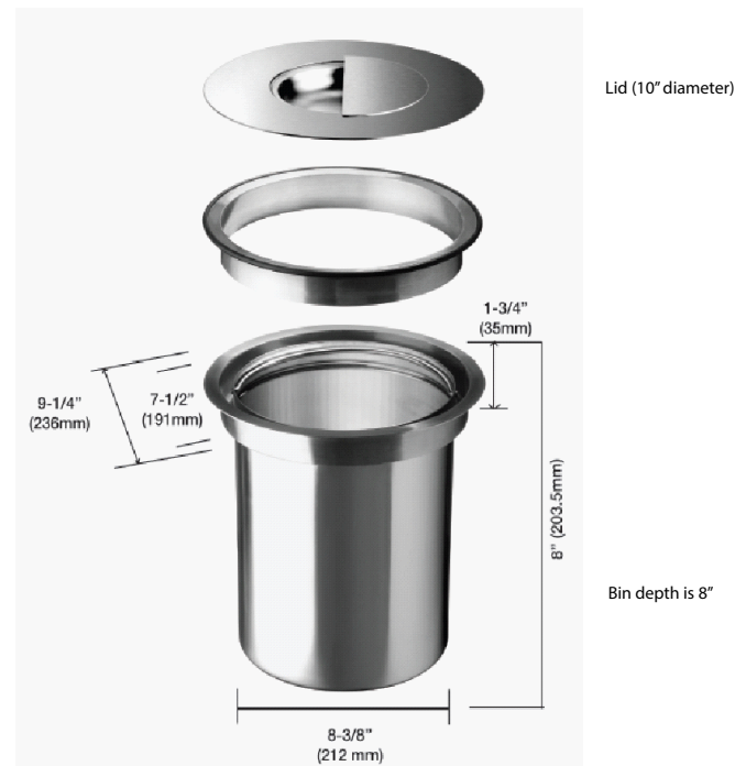
Drop-in installation
